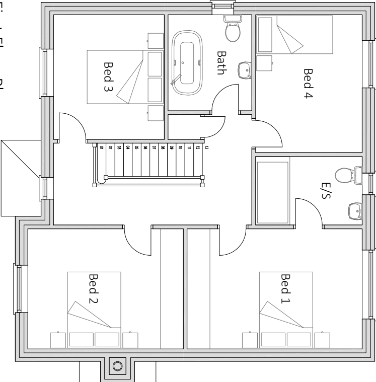
First Floor Plan GIFA - 73.3 sqm
