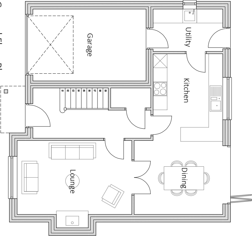
Ground Floor Plan GIFA - 74.1 sqm
