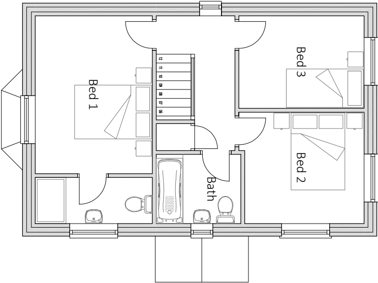
First Floor Plan GIFA - 46.3sqm
