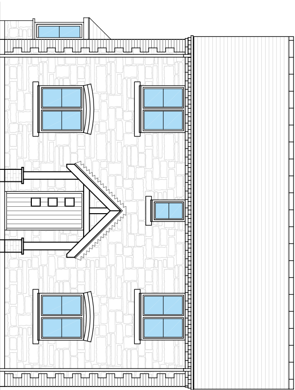
Front Elevation
