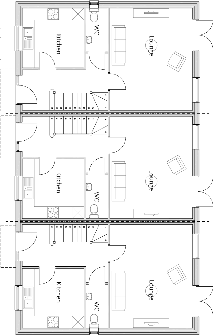
Ground Floor Plan GIFA - 44 sqm
