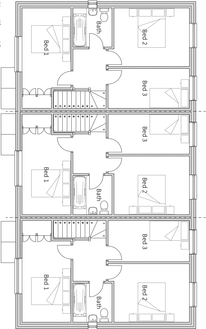
First Floor Plan GIFA - 44 sqm
