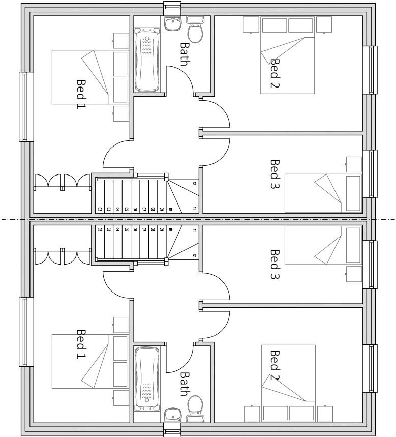
First Floor Plan GIFA - 44 sqm
