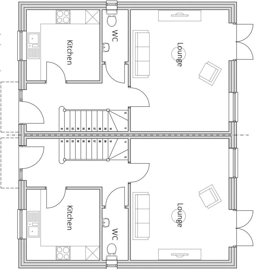
Ground Floor Plan GIFA - 44 sqm
