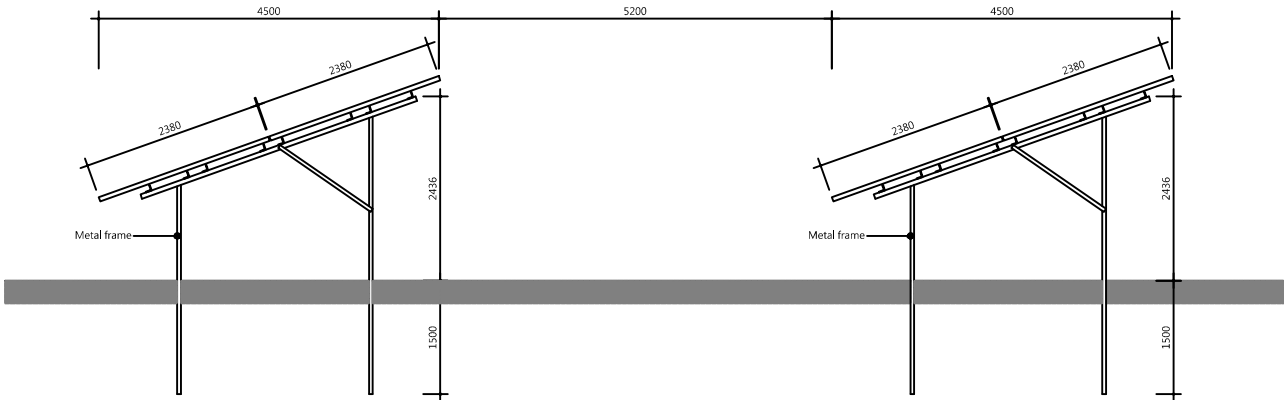
SIDE ELEVATION
