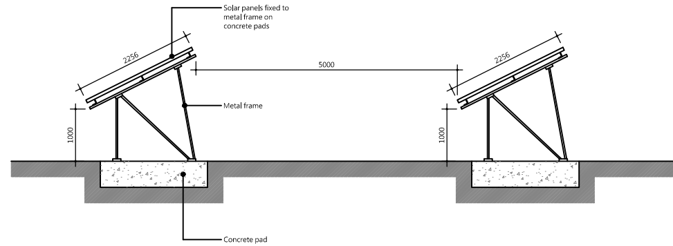
SIDE ELEVATION
