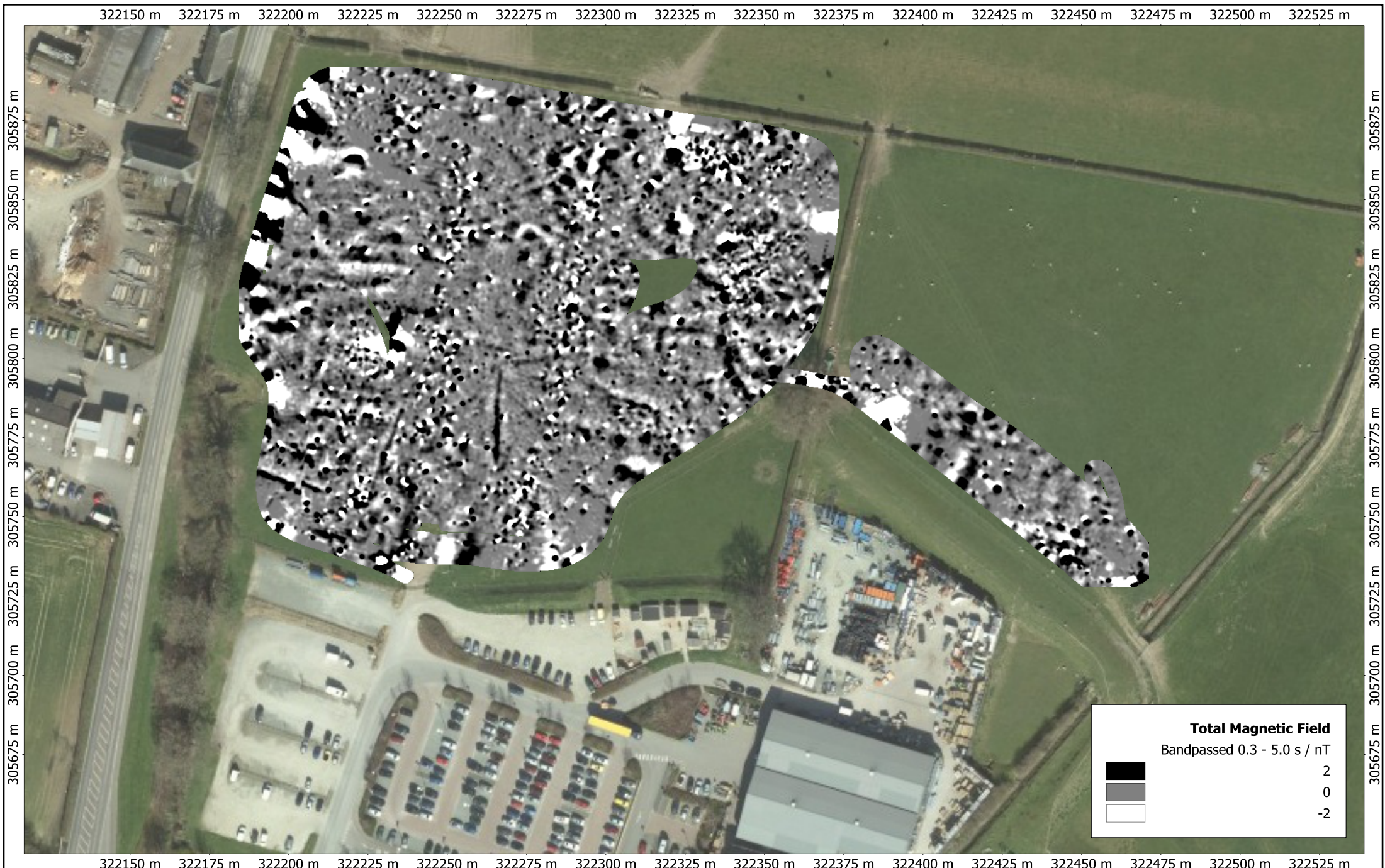
SSW151 Land South of Welshpool, Powys DWG 02 Magnetic Data Plot
