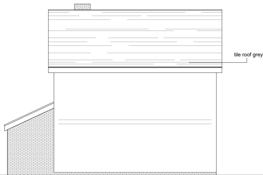
Side Elevation
