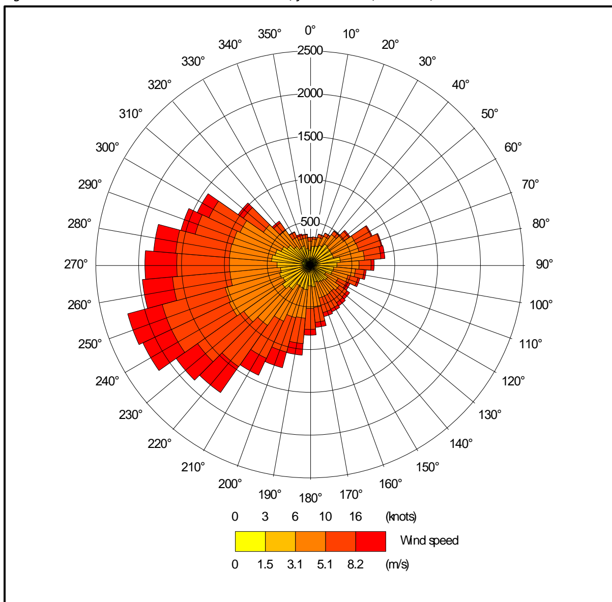
Figure 2a. The wind rose. Raw GFS derived data, for 52.314 N, 3.496 W, 2014 – 2017
