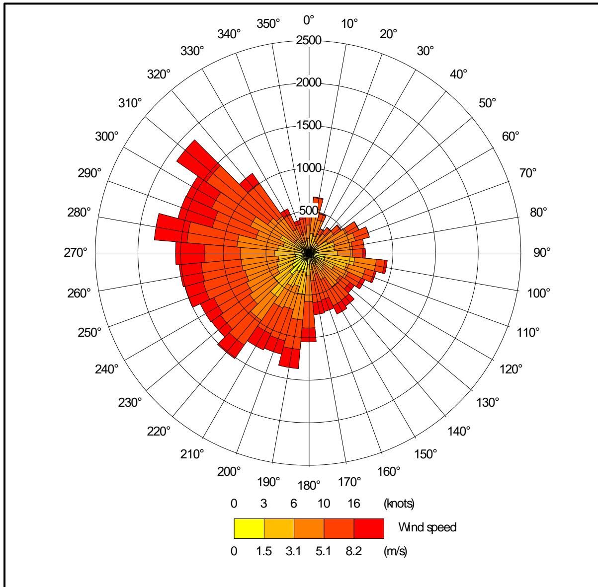
Figure 2b. The wind rose. FLOWSTAR modified GFS derived data for NGR 298000, 269550, 2014-2017
