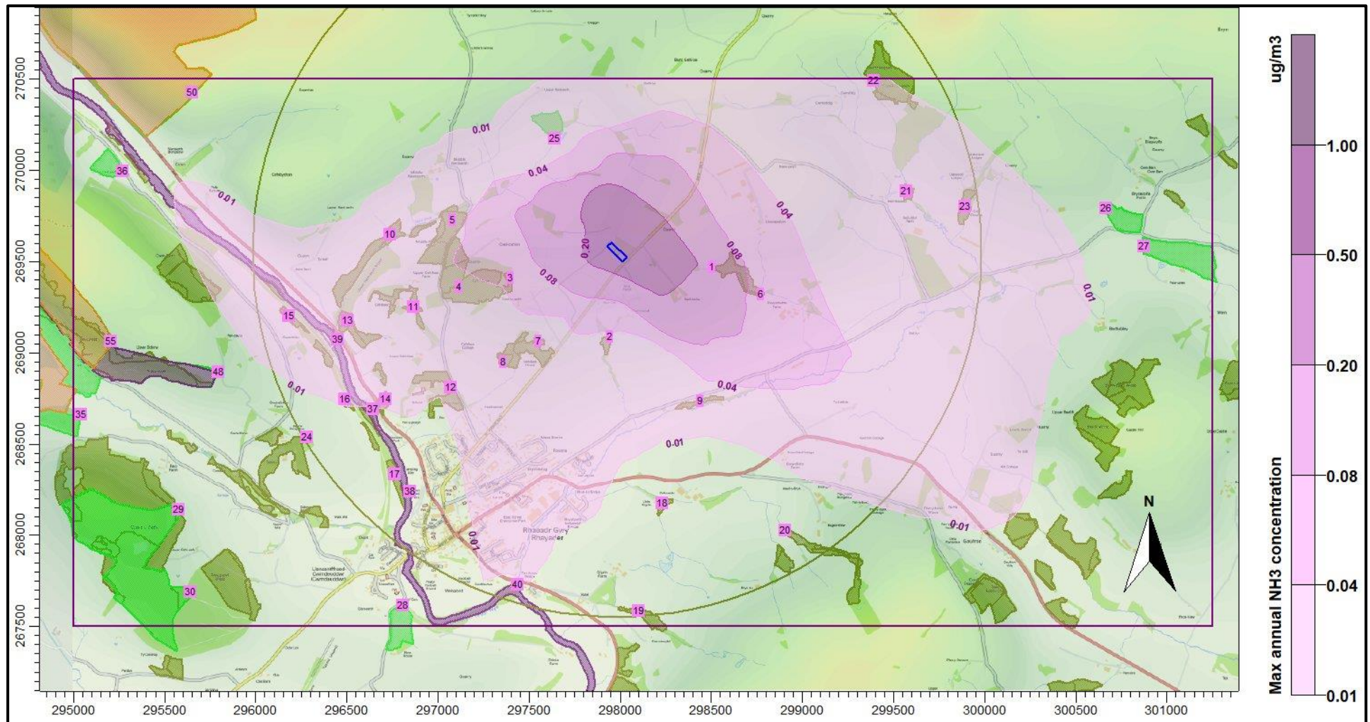
Figure 6. Maximum annual ammonia concentration
