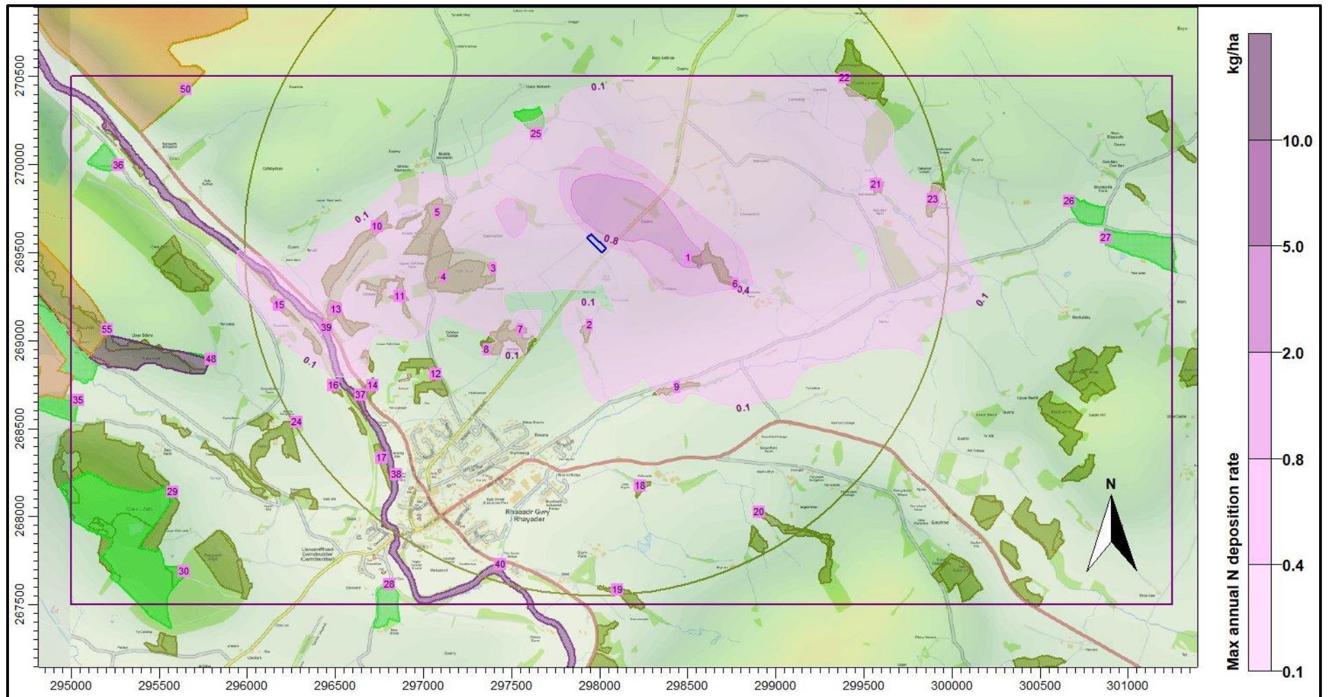
Figure 7. Maximum annual nitrogen deposition rates
